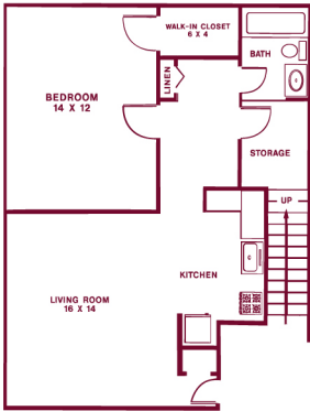
1-BEDROOM STANDARD FIRST FLOOR
