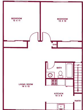
2-BEDROOM STANDARD SECOND FLOOR
